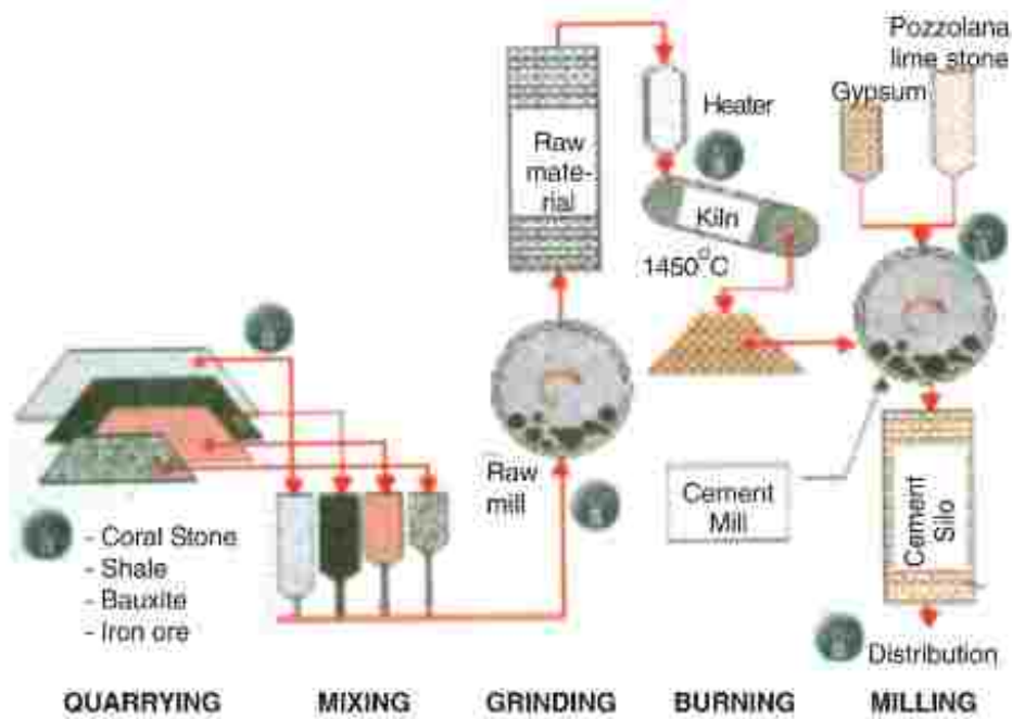
Fig-1 Process of cement production
