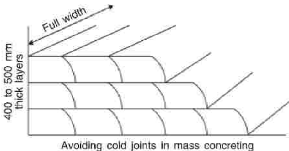
Fig - 4 Step Placing in Concrete
