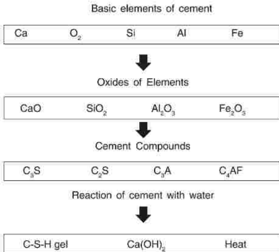
Fig-2 Reaction of cement with water
