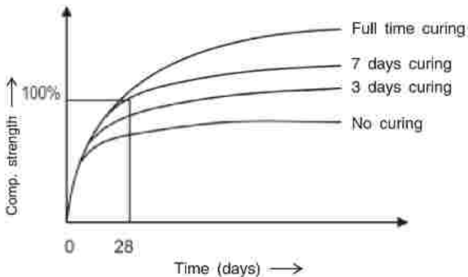
Fig-4 Effect of curing
