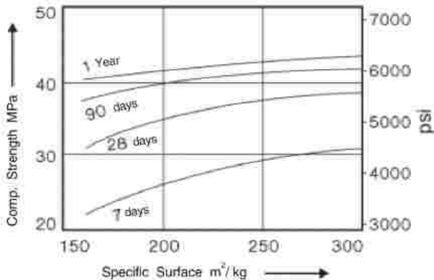
Fig - 3 Relation between specific surface and strength
