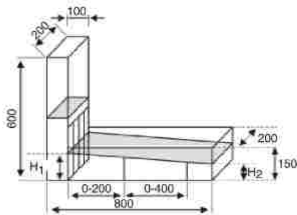
Fig-3 L - Box Test
