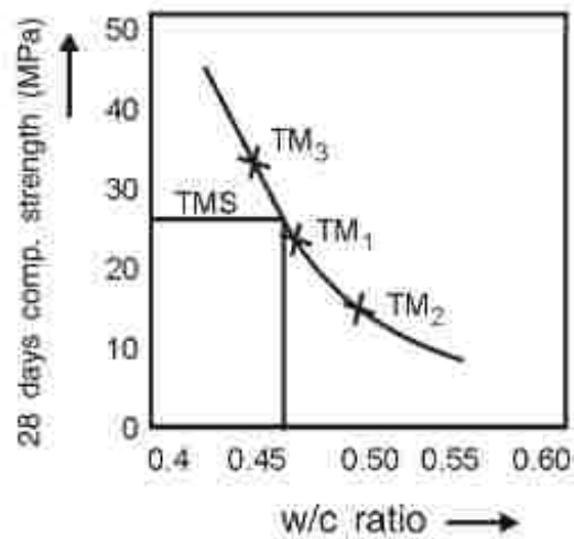
Fig-4 Strength v/s w/c ratio
