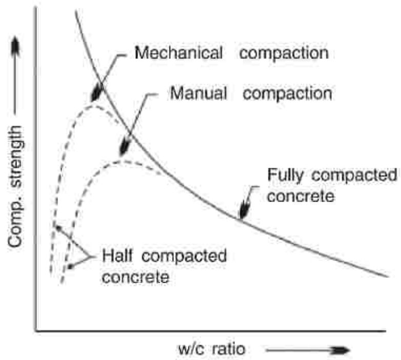
Fig - 5 Importance of Compaction
