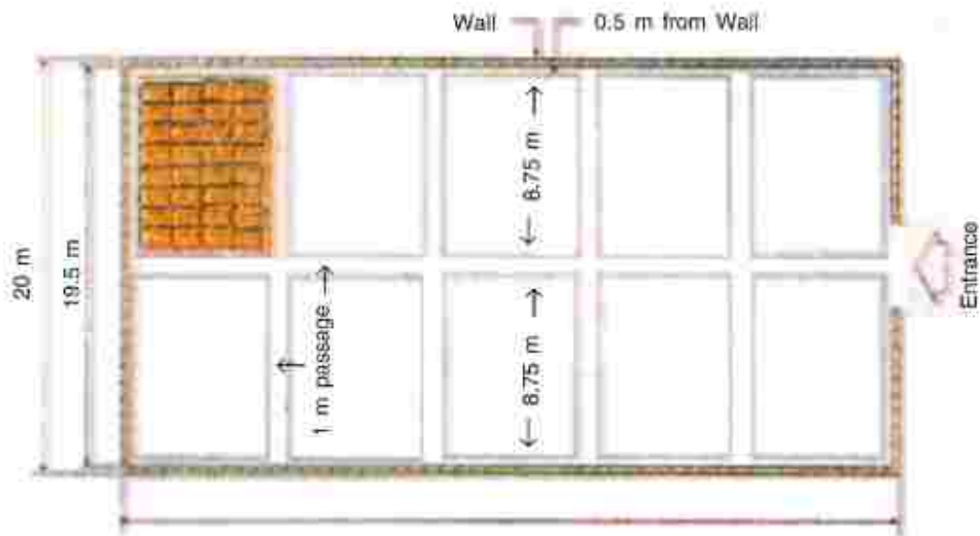
Fig - 7 Cement storage
