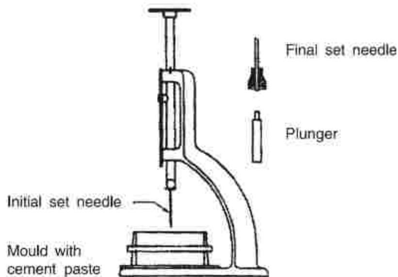
Fig - 4 Vicat's Apparatus
