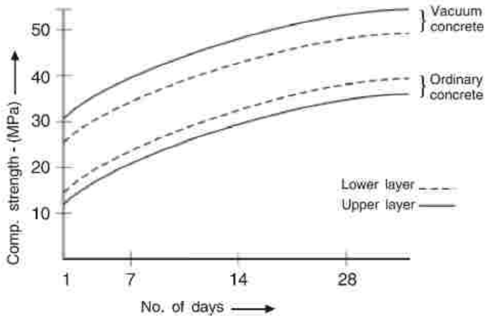
Fig - 6 Effect of de-watering
