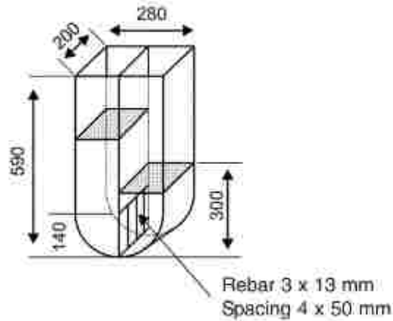
Fig 2 U - Flow test
