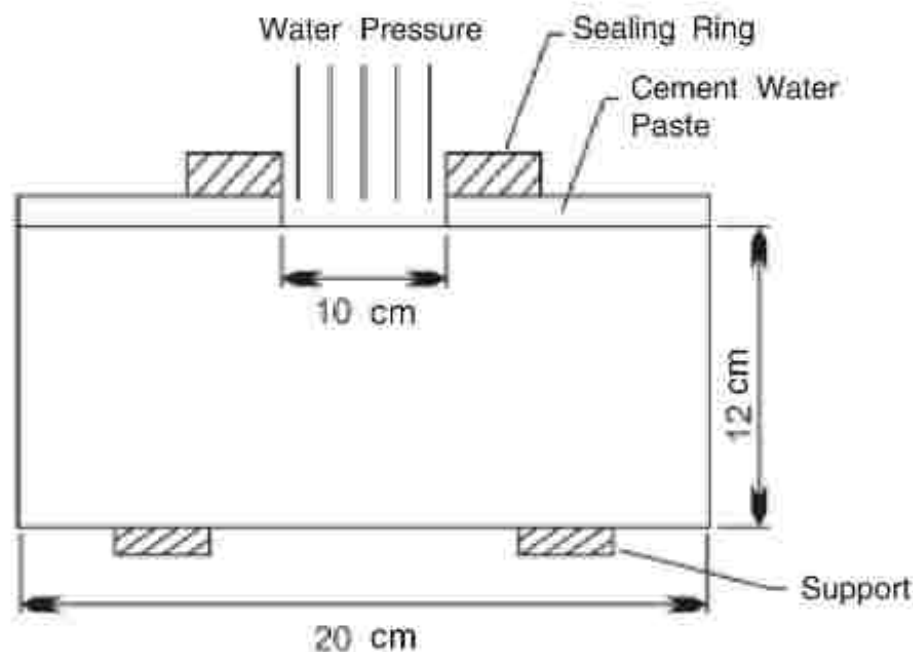
Fig - 3 Permeability Test
