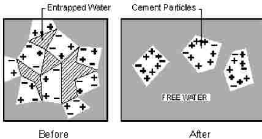
Fig - 1 Physical Interaction of Super-Plasticizer
