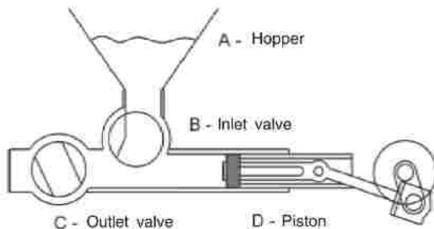
Fig - 2 Concrete Pump
