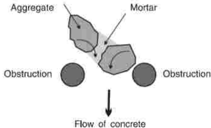
Fig - 1 Friction between the particles
