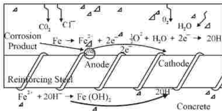
Fig-2 Electro-chemical Process of Corrosion
