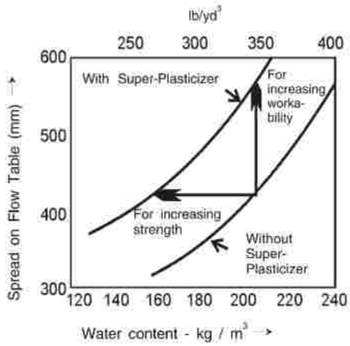
Fig - 2 Effect of Super-Plasticizer
