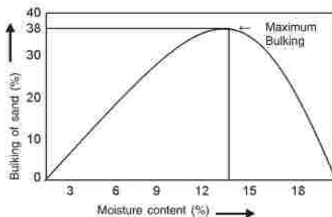
Fig - 2 Bulking of sand
