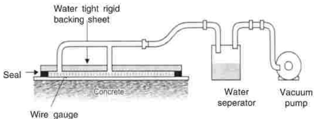
Fig - 5 Vacuum Dewatering
