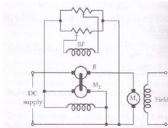
Fig.16 Booster control
