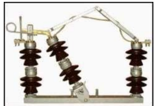
Figure1.1: AIR BREAK SWITCH
