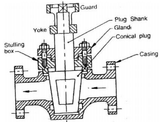
Fig. 3.10 Blow off cock
