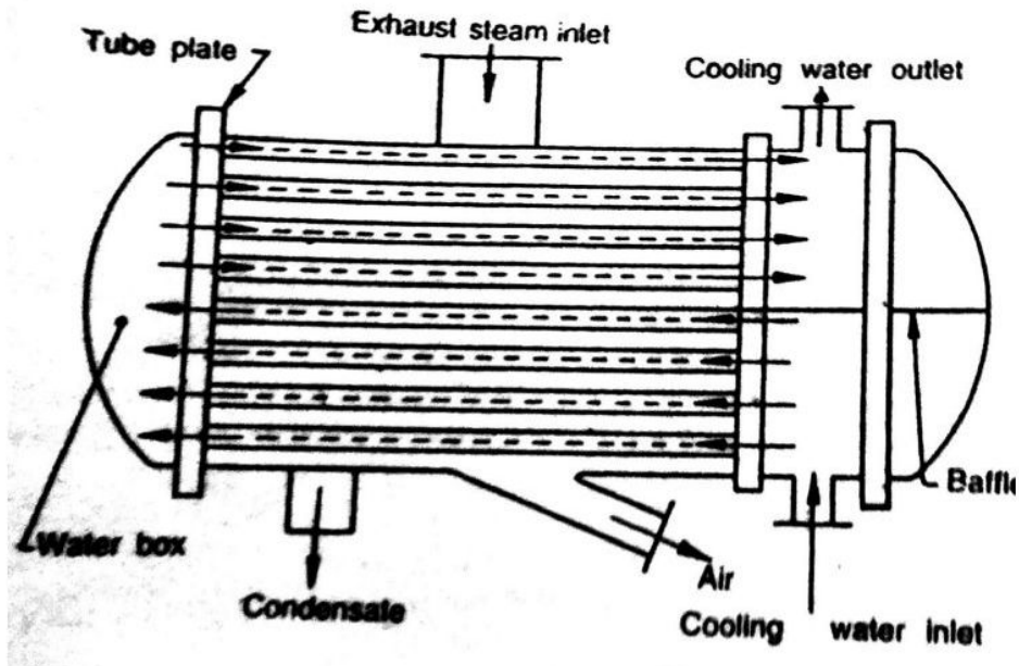
Fig. 6.5 Surface Condensers
