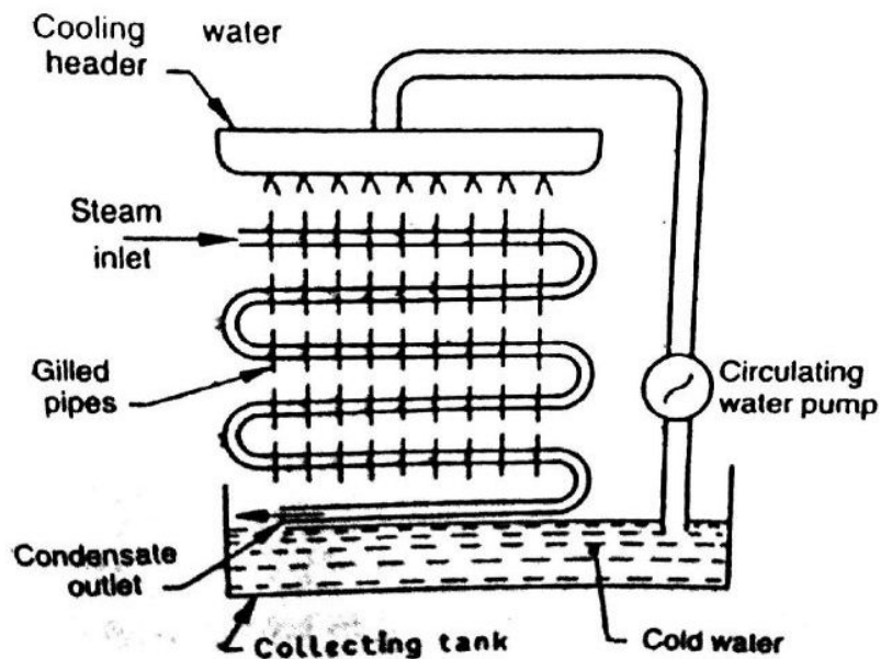
Fig. 6.8 Evaporative Condenser
