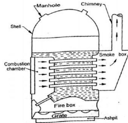
Fig. 3.1 Cochran Boiler
