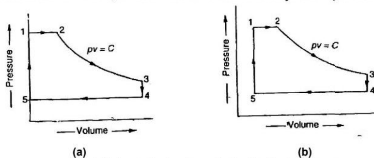
Fig. 4.3 Theoretical or hypothetical indicator diagram
