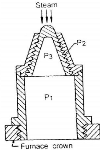
Fig. 3.12 Fusible plug
